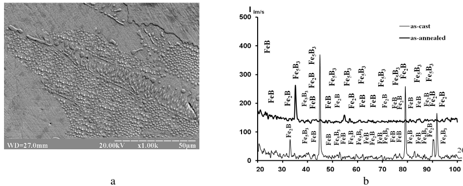
Fig. 4. Fe-B alloy with boron content of 9.3 wt. %: microstructure (a) after annealing at 1473 K for 4 hours and after cooling with the rate of 10^2 K/s; as-cast and as-annealed diffractograms (b).
