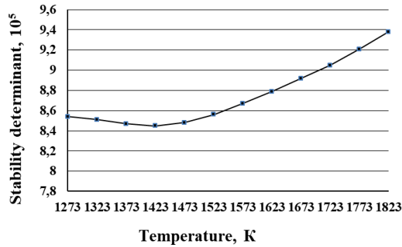
Fig. 5. Temperature dependence of the determinant of thermodynamic stability for FeB monoboride.
