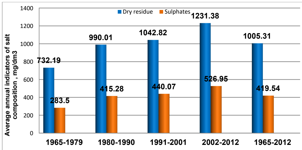
Fig. 3. Levels of average annual indicators salt composition of drinking water in Karachunovskyi reservoir in 1965-2012 years ( M \pm m ), \text{mg}/\text{dm}^3 .
